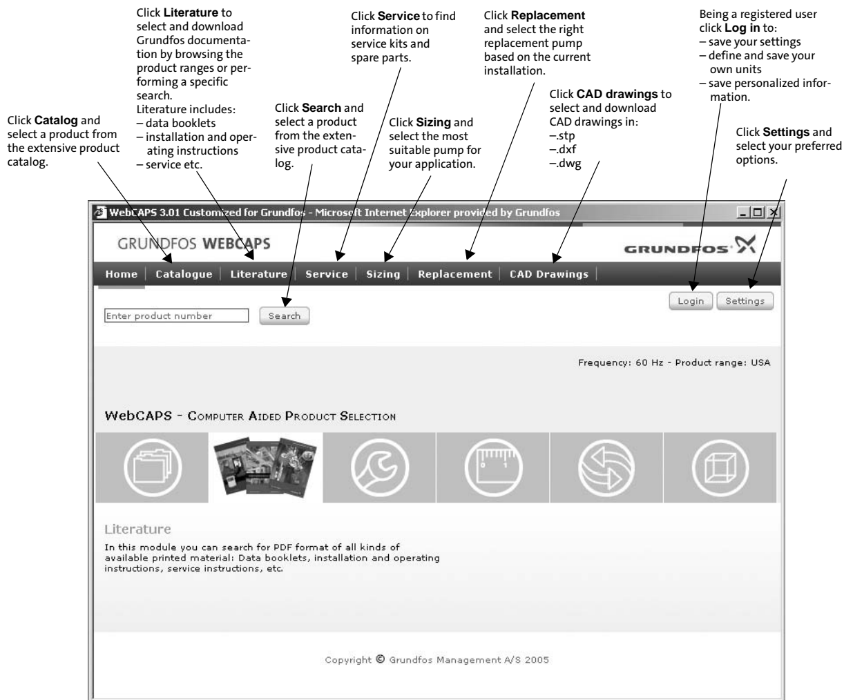
Fig. 31 WebCAPS
