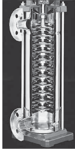
Top and bottom suction/discharge design
